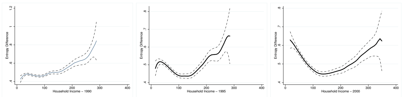
Figure 7: Estimated differences with confidence intervals
