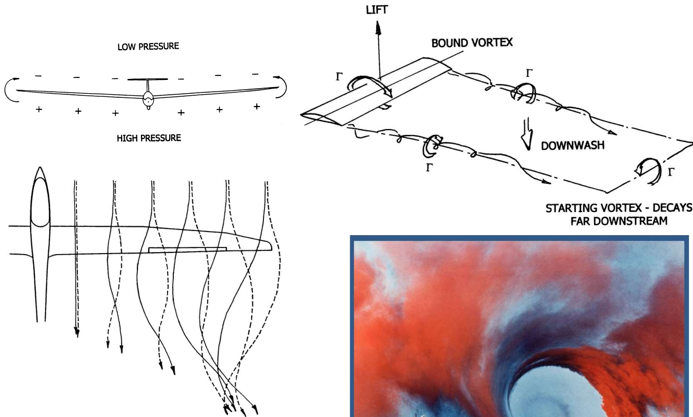
Fig. 2 Spanwise flow on a finite wing - solid lines, upper surface; dashed lines, lower surface.
