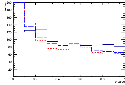
(b) 1st order Chebychev polynomial
