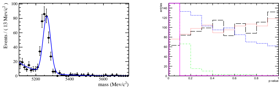
Figure 25: The B^0 invariant mass distribution is shown for a toy experiment (left), when the fixed Gaussian mean of the fit function is shifted by 10 \text{MeV}/c^2 . The corresponding p-value distribution is shown on the right. The black line corresponds to a shift of 1 \text{MeV}/c^2 , the blue line corresponds to 2 \text{MeV}/c^2 , the red line correspond to 5 \text{MeV}/c^2 , the green line corresponds to 10 \text{MeV}/c^2 and the purple line corresponds to 20 \text{MeV}/c^2 .
