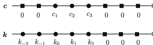
Figure 1: Vectors \vec{c} and \vec{k} used for the convolution
