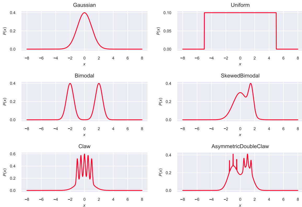
Figure 2: Test distributions used to sample data from
