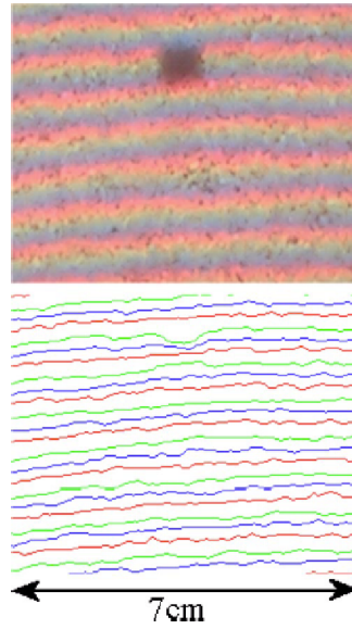
Fig. 3. (top panel) Detail of the set of colored lines projected onto the pile. (bottom panel) The centre of gravity of the lines as recognized by the software.
