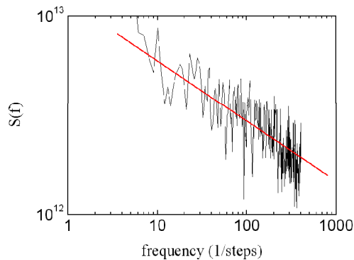
Fig. 10. Powerspectrum of the avalanches of figure 6. The red line indicates power-law behavior with a negative power of 0.27(3) , very close to the value of the growth exponent, 0.28(3) , in good agreement with SOC theory.
