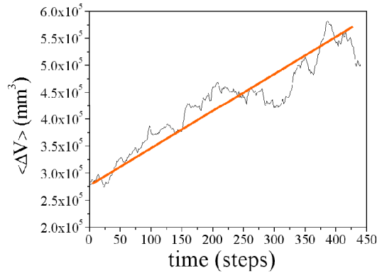
Fig. 13. Size of the avalanches of figure 12 averaged over 100 time steps. Clearly the average avalanche size increases linearly with time while the system is developing towards the SOC steady state.
