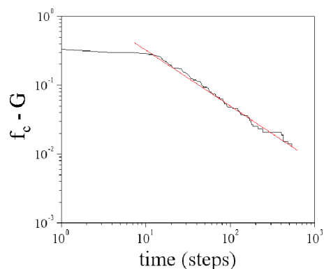
Fig. 14. Difference between actual maximal slope anywhere in the pile G and the critical slope f_c of rice as a function of time. The red line indicates power law behavior with slope 0.8(1).
