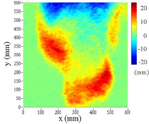
Fig. 5. Typical avalanche on the rice pile. The picture shows the avalanche as the difference in height between two successive images.
