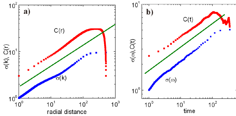
Fig. 4. (a) Determination of the roughness exponent from the spatiotemporal correlation function C(L, 0) and the distribution function \sigma(k) as defined in the text. The line indicates the average slope, which defines the value for the roughness exponent obtained. (b) Determination of the growth exponent from the spatiotemporal correlation function C(0, t) and the distribution function \sigma(\omega) as defined in the text. The line indicates the average slope, which defines the value for the growth exponent obtained
