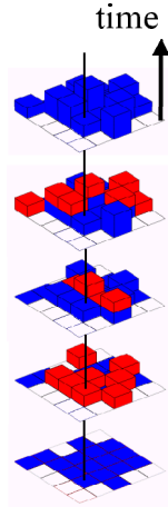
Fig. 9. Schematic representation of the spatiotemporal structure of an avalanche. Shown are five successive stages of development of an avalanche cluster, shown in full-grown state at the top. At the bottom the substrate area of the full-grown avalanche is shown. As time progresses there is activity (red) or not (blue) at a particular site. A time line running through one site is indicated by the vertical line. For further explanation see text.
