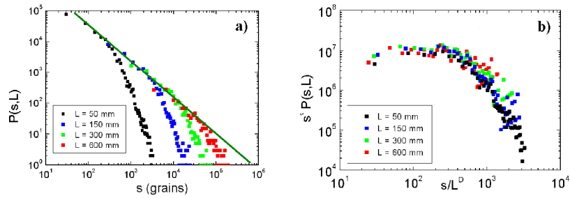
Fig. 7. (a) Size distribution of the avalanches. P(s, L) is the number of avalanches of size s that were observed while monitoring a window of size L \times L (b) Finite size scaling of the size distribution of the avalanches. Note the nice data-collapse: the deviation from powerlaw behavior starts from a size s \sim L^D where D is the fractal dimension of the avalanche volume.
